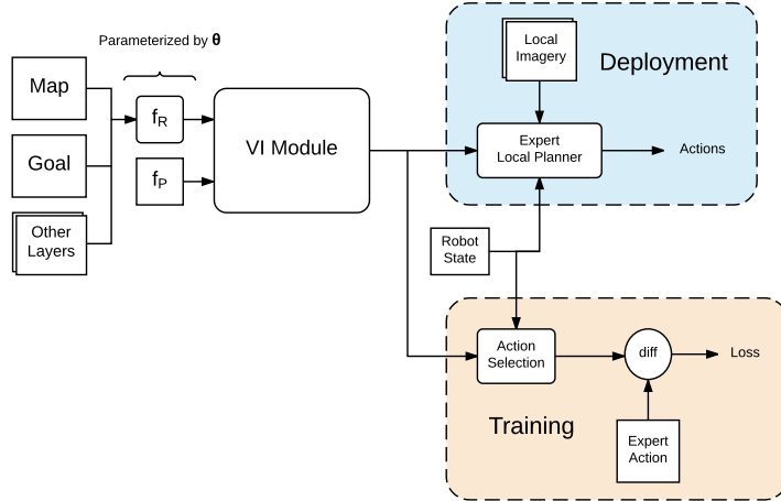
Figure 2: Information flow diagram for our architecture.
